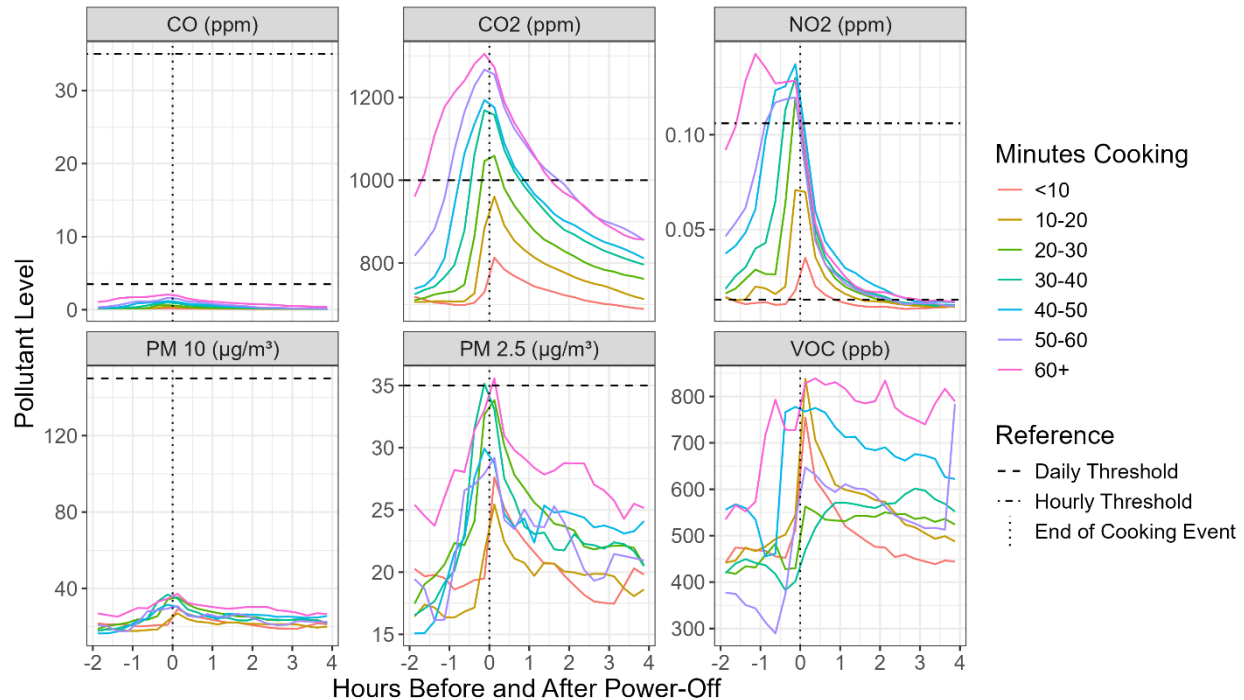
Figure 3: Average cooking event timeseries with gas ranges only, by cooking event length, with health thresholds overlaid; in the case of multiple applicable thresholds, the least strict is shown 3
