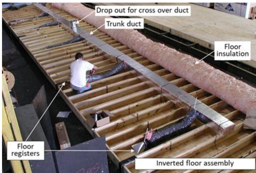
Figure 13. Duct system being installed on an inverted floor section that will be flipped over once completed
