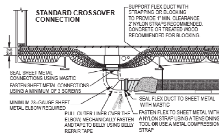
Figure 9. Cross-over connection specifications for the Northwest Energy-Efficient Manufactured Housing Program.
