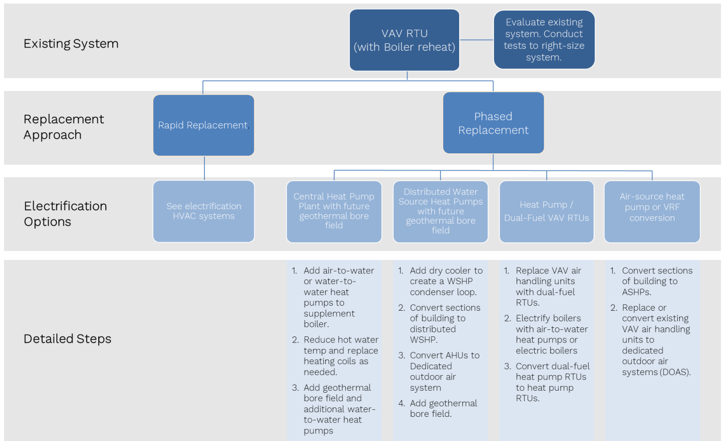
Figure 15. VAV RTU (with boiler reheat) electrification replacement options
