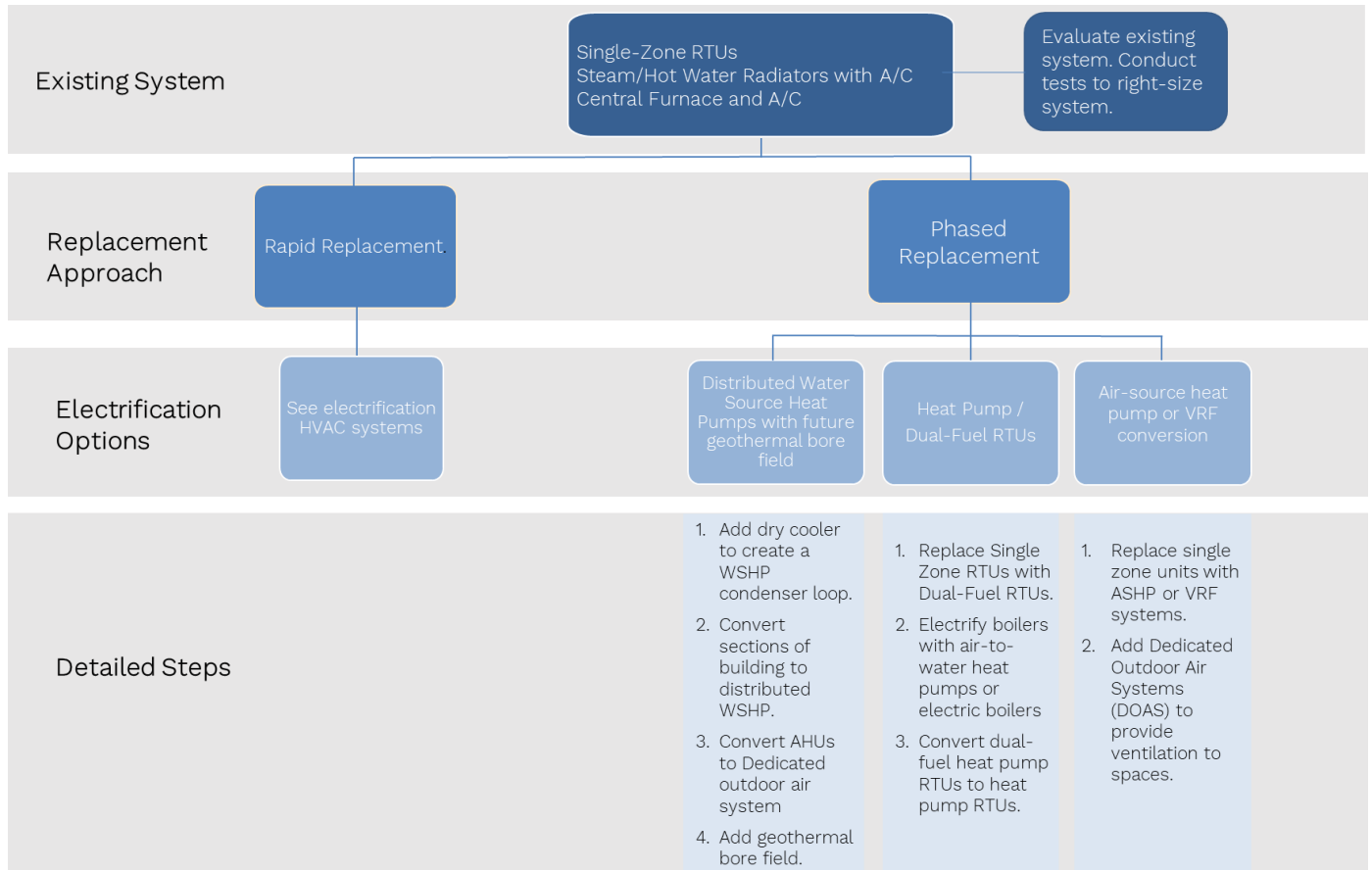
Figure 16. Single-zone RTUs, steam/hot water radiators, central furnaces with ACs electrification replacement options
