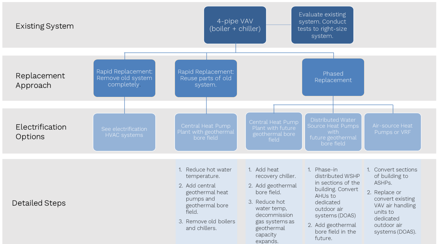
Figure 14. 4-pipe VAV boiler and chiller system electrification replacement options
